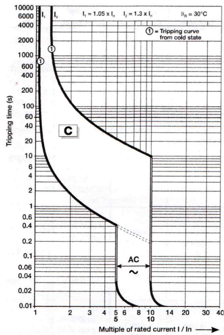
C Curve
