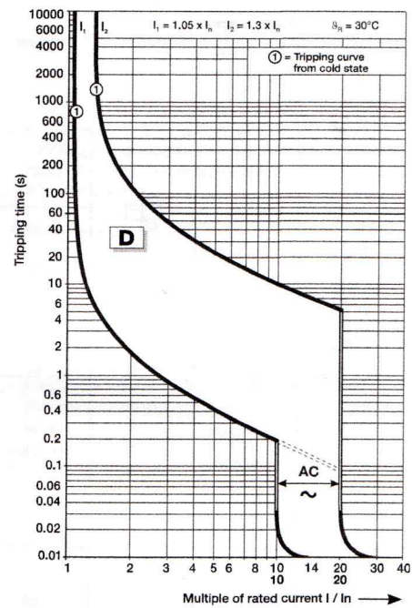
D Curve
